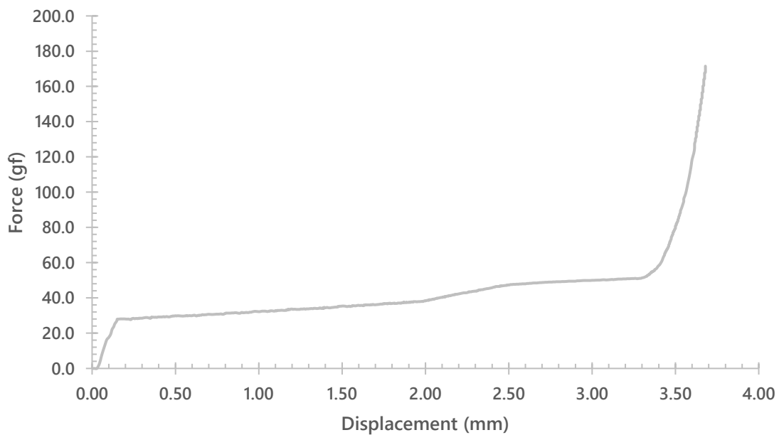
Gateron Oil King Silent Linear (Upstroke)
